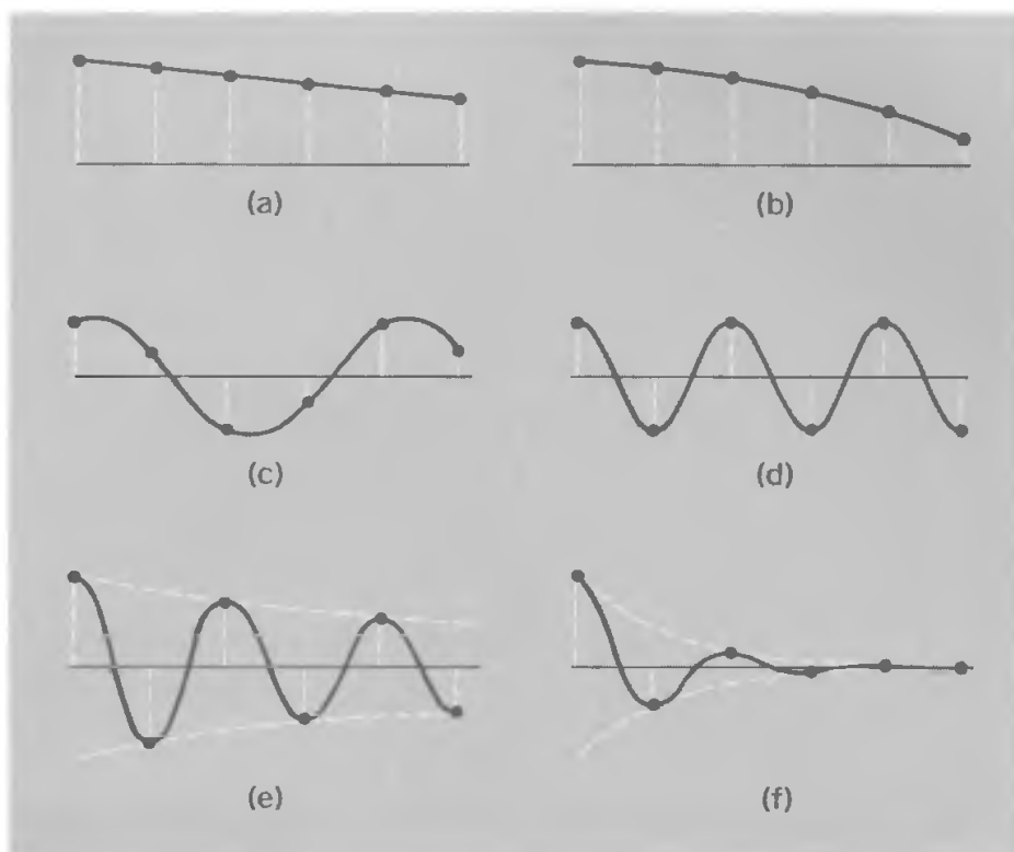
Fig. 7-17 Amplitude relationships for particles on a string, driven at left end. (a) Static equilibrium, \nu = 0 . (b) \nu \ll \nu_0 . (c) \nu = \sqrt{2}\nu_0 . (d) Highest mode, \nu = 2\nu_0 . (e) \nu > 2\nu_0 . (f) \nu \gg 2\nu_0 .
