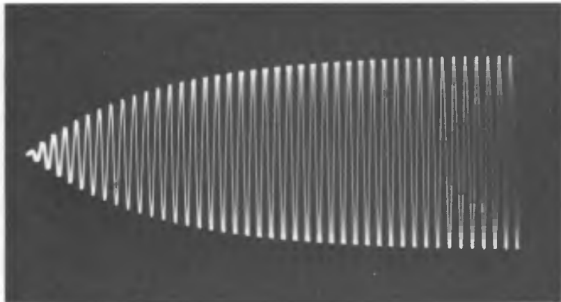
Fig. 4-11 (a) Response of an undamped harmonic oscillator to a periodic driving force, as described by Eq. (4-19). This beat pattern would continue indefinitely. (b) Transient behavior of a damped oscillator with a periodic driving force off resonance. (c) Transient behavior at exact resonance, showing smooth growth toward steady amplitude. (Photos by Jon Rosenfeld, Education Research Center, M.I.T.)
