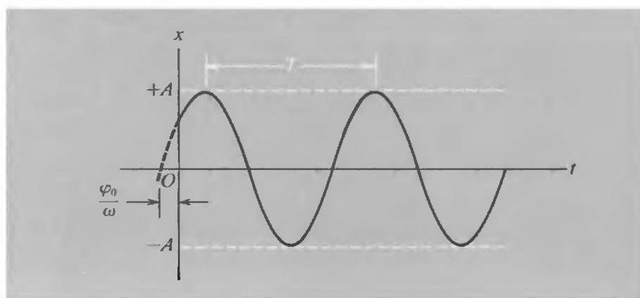
Fig. 1-2 Simple harmonic motion of period T and amplitude A .
