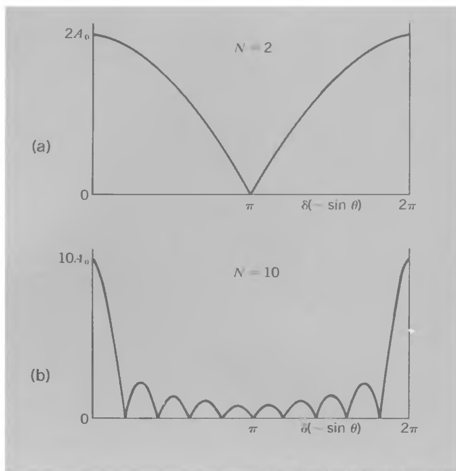
Fig. 8-20 (a) Variation of amplitude with phase difference for two-slit interference. (b) Variation of amplitude with phase difference for ten-slit interference.
