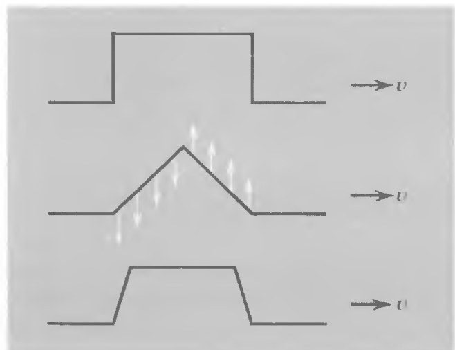
Fig. 7-16 Geometrical idealizations of simple types of pulse.
