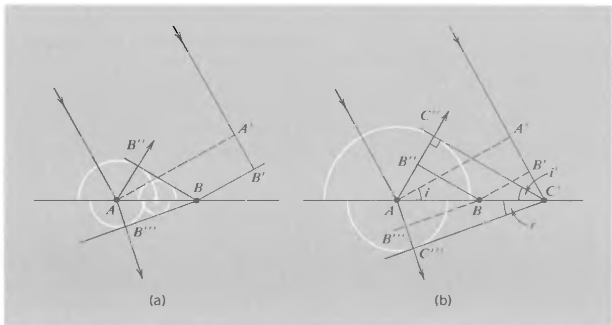
Fig. 8-9 (a) Reflection and refraction by Huygens' construction. (b) Proof of Snell's Law by Huygens' construction.
