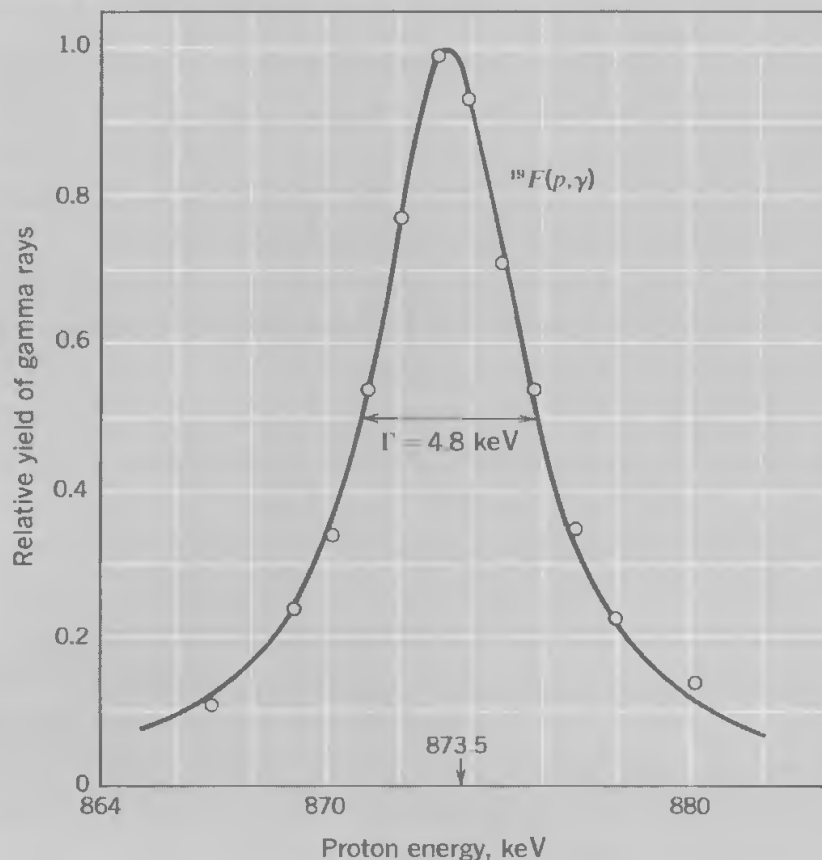
Fig. 4-16 Yield of gamma rays as a function of the energy of bombarding protons in the reaction p + {}^{19}\text{F} \rightarrow {}^{20}\text{Ne} + \gamma . [From data of R. G. Herb, S. C. Snowden, and O. Sala, Phys. Rev., 75, 246 (1949).]
