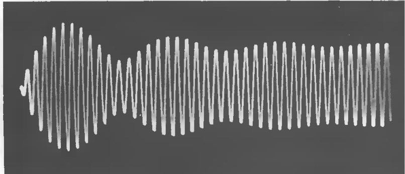
Fig. 4-11 (a) Response of an undamped harmonic oscillator to a periodic driving force, as described by Eq. (4-19). This beat pattern would continue indefinitely. (b) Transient behavior of a damped oscillator with a periodic driving force off resonance. (c) Transient behavior at exact resonance, showing smooth growth toward steady amplitude. (Photos by Jon Rosenfeld, Education Research Center, M.I.T.)
