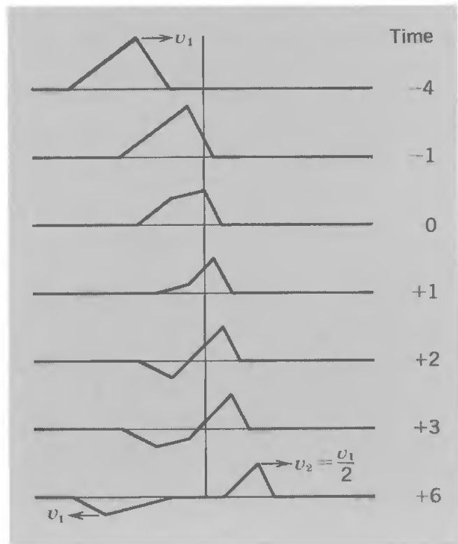
Fig. 8-3 Partial reflection and transmission of triangular wave pulse at the junction of two strings. Pulse is incident from string with higher wave speed. ( v_2 = \frac{1}{2}v_1 .)
