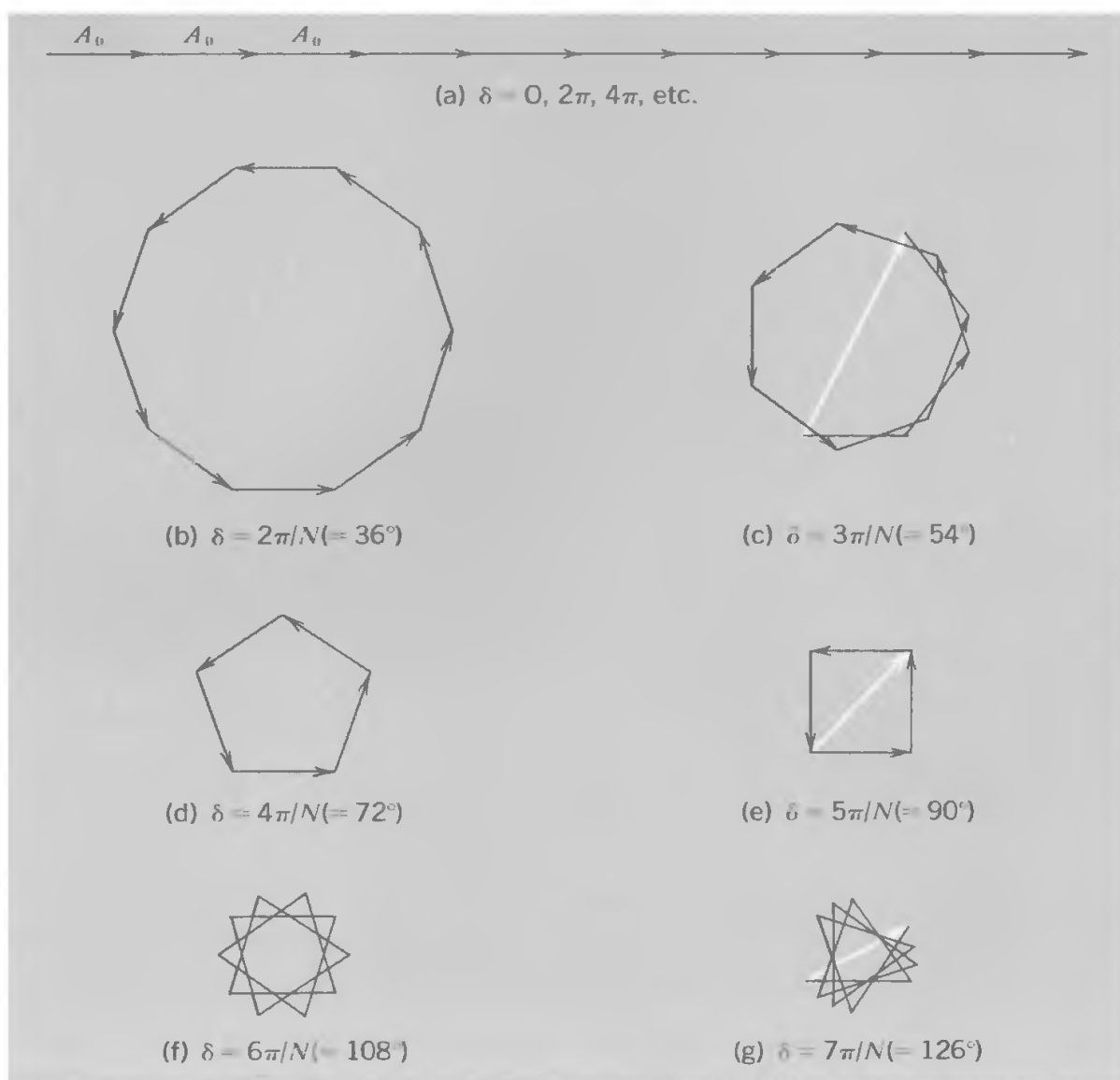
Fig. 8-19 Vector diagrams for diffraction grating ( N = 10 ). (a) \delta = 0, 2\pi, 4\pi, \text{ etc.} (b) \delta = 2\pi/N (= 36^\circ) . (c) \delta = 3\pi/N (= 54^\circ) . (d) \delta = 4\pi/N (= 72^\circ) . (e) \delta = 5\pi/N (= 90^\circ) . (f) \delta = 6\pi/N (= 108^\circ) . (g) \delta = 7\pi/N (= 126^\circ) .
