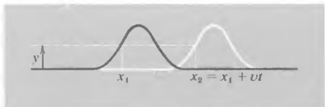
Fig. 7-12 Movement of an arbitrary traveling pulse.
