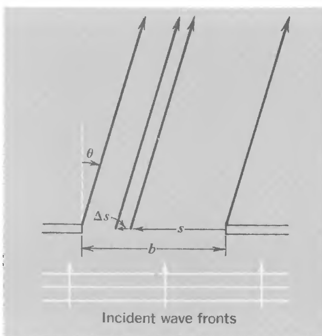
Fig. 8-22 Single-slit diffraction.
