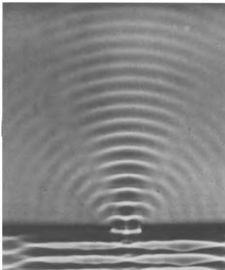
Fig. 8-25 Single-slit diffraction of water waves. (From the film "Ripple Tank Phenomena," Part II, Education Development Center, Newton, Mass.)
