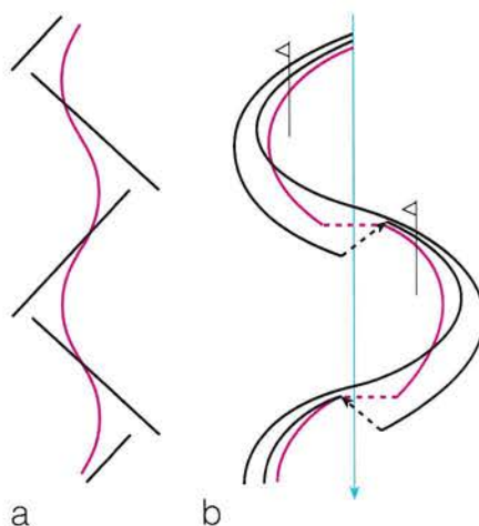
Figure 10. The skating technique on a flat site (a) and on a slope (b). The red curves are the trajectories of the skier's center of mass, while the black curves are the tracks of the skis.
