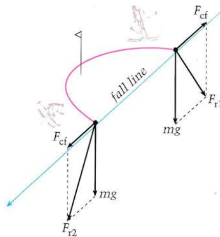
Figure 12. The resultant of the gravitational and centrifugal forces at the beginning and the end of an arc: F_{r2} > F_{r1} .
