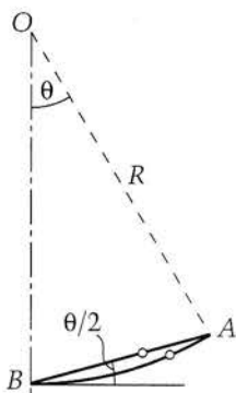
Figure 4. Beads on wires. The time required to slide down along the arc AB is shorter than that along the subtending chord.
