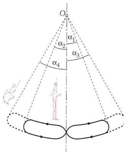
Figure 11. Trajectory of the center of mass during swinging on a swing.
