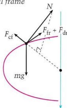
Figure 2. Inertial and noninertial reference frames. A centrifugal force acts on the skier in the noninertial reference frame. Here and in the following figures the blue arrows denote the direction of the fall line.
