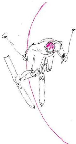
Figure 6. Snowplow (or wedge) turn: Standing on the inside ski, the skier pushes against the snow with the outside ski.
