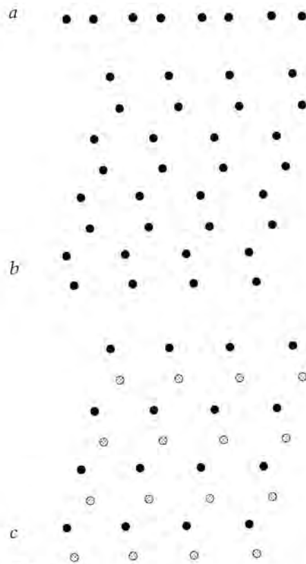
Figure 8 Regular systems of points: (a) one-dimensional, (b) two-dimensional, (c) decomposition of a regular system into lattices.
