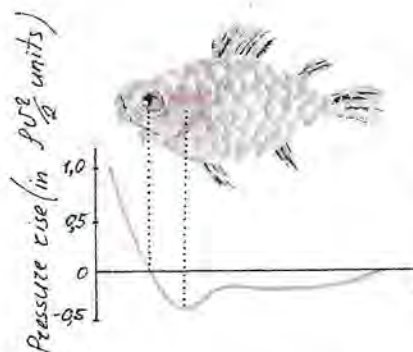
Figure 7 Distribution of pressure around the body of a swimming fish.
