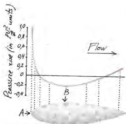
Figure 4 Distribution of pressure in a fluid flowing around a symmetrical drop-shaped body. (Since the variation in pressure is always proportional to \rho v^2/2 , it can be expressed in dimensionless units 2p/\rho v^2 .)
