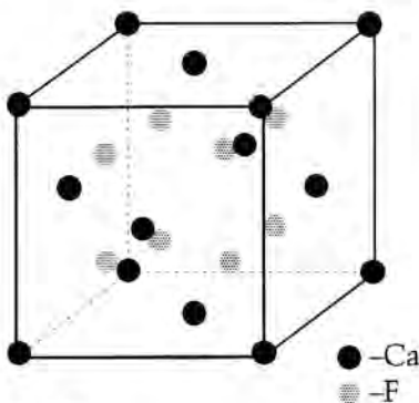
Figure 9 Structure of fluorite, composed of two different regular systems (the gray dots are fluorine atoms, black are calcium).
