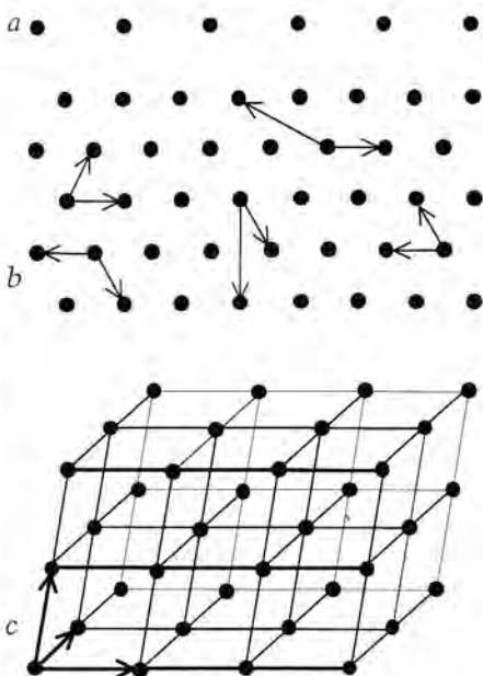
Figure 5 Types of lattices: (a) one-dimensional, (b) two-dimensional (plane), (c) three-dimensional. Arrows show the base vectors of coordinate systems defining the lattices.
