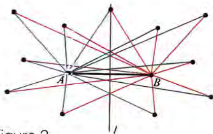
Figure 3 Part of a symmetric Delone system. Its only nonidentical symmetry transformation is the reflection in line l . Points A and B have congruent global stars.
