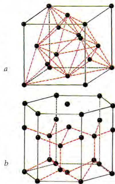
Figure 10 Structure of (a) diamond, (b) lonsdalite.
