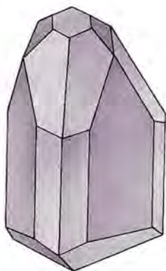
Figure 7 Tourmaline crystal.
