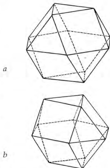
Figure 11 Second coordinate spheres in (a) diamond, (b) lonsdalite.
