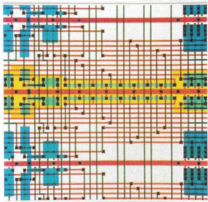
Diagram of "CRISP" microprocessor by AT&T Bell Laboratories
