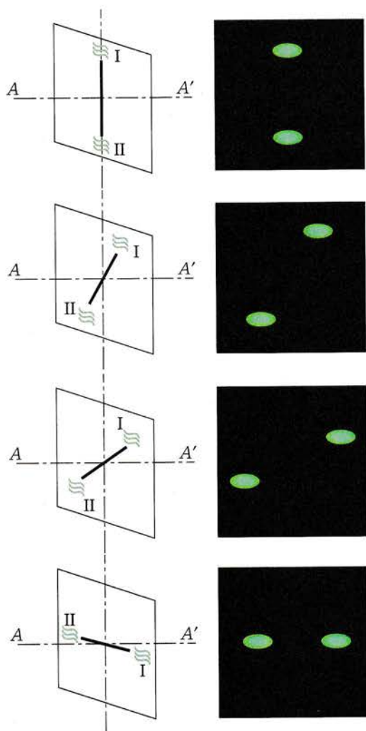
Figure 4 Photographs of light dumbbells oriented differently relative to the camera's line of sight. The exposure time is 10^{-11} s.
