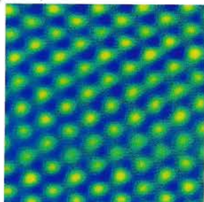
Graphite Atoms
