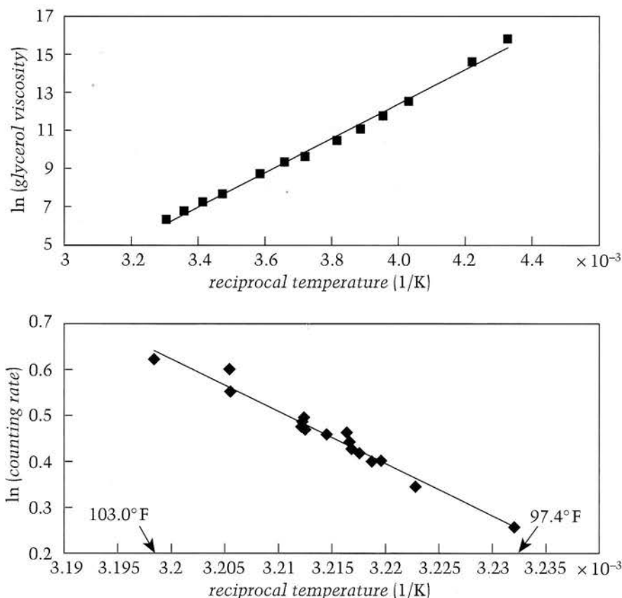
Figure 3 Arrhenius plot of glycerol viscosity and counting rate.
