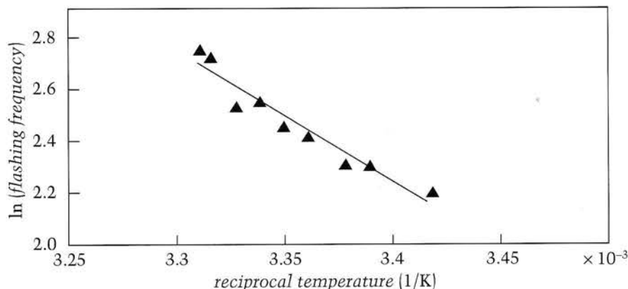
Figure 2 Arrhenius plot for frequencies of cricket chirping and firefly flashing.
