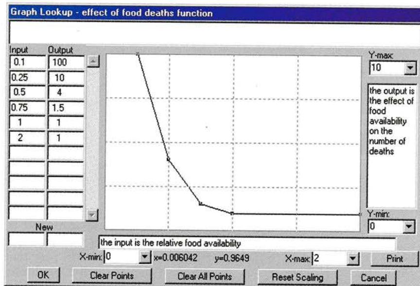
Figure 4 The "effect of food deaths" function.
