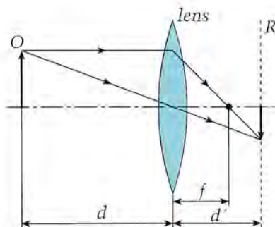
Figure 1. Formation of an image on the retina of an eye. Shown are the object O, lens, and retina R.
