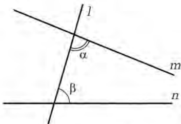
Figure 1. In the figure, if \angle \alpha + \angle \beta < 180^\circ , then lines m and n will intersect to the right of line 1.
