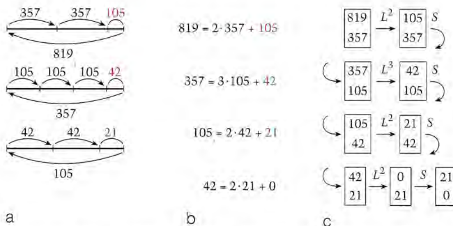
Figure 3. To find \text{GCD}(819, 357) = 21 using Euclid's algorithm, four steps are needed.
