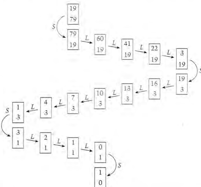
Figure 4. Every "flight of stairs" of this staircase represents one step of Euclid's algorithm.
