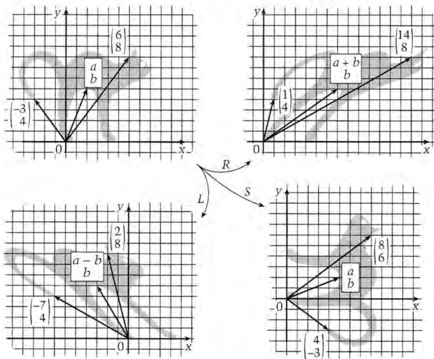
Figure 6. "Left skew" L(x, b) \rightarrow (x - b, b) , "right skew" R(x, b) \rightarrow (x + b, b) , and "symmetry" S(x, b) \rightarrow (b, x) are linear transformations that perform one-to-one mappings of the integer lattice \mathbb{Z}^2 onto itself.
