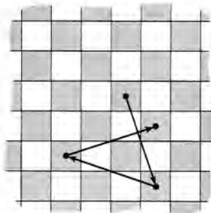
Figure 1. The \{1, 3\} -knight can reach any diagonally adjacent square: these elementary steps can be used to visit all squares of the same color.
