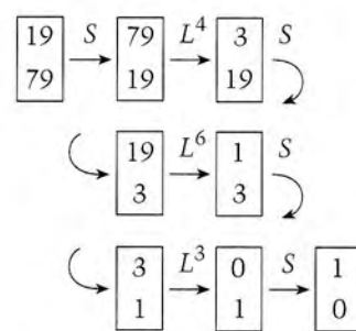
Figure 2. The numbers 19 and 79 are relatively prime (they are called coprimes); therefore, several divisions with remainder give the remainder 1 = \text{GCD}(19, 79) .
