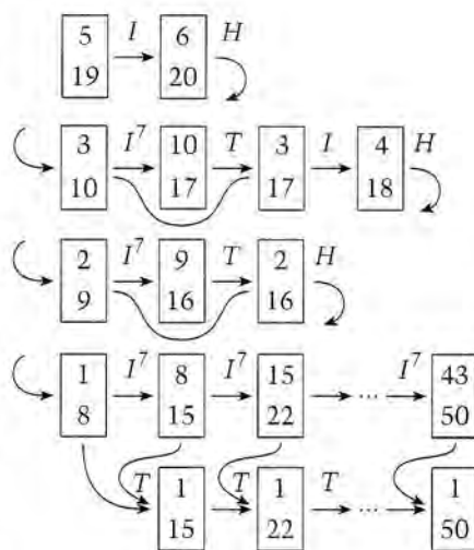
Figure 7. Using the operations I^q (increment by q ), H (division by two), and T (transitive transformation), we can obtain card (1, 50) from (5, 19).
