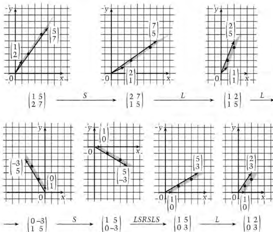
Figure 9. Reduction to the canonical form. Under all transformations L , R , and S , the area of the parallelogram and the location of the nodes of the integer lattice inside the parallelogram remain the same.
