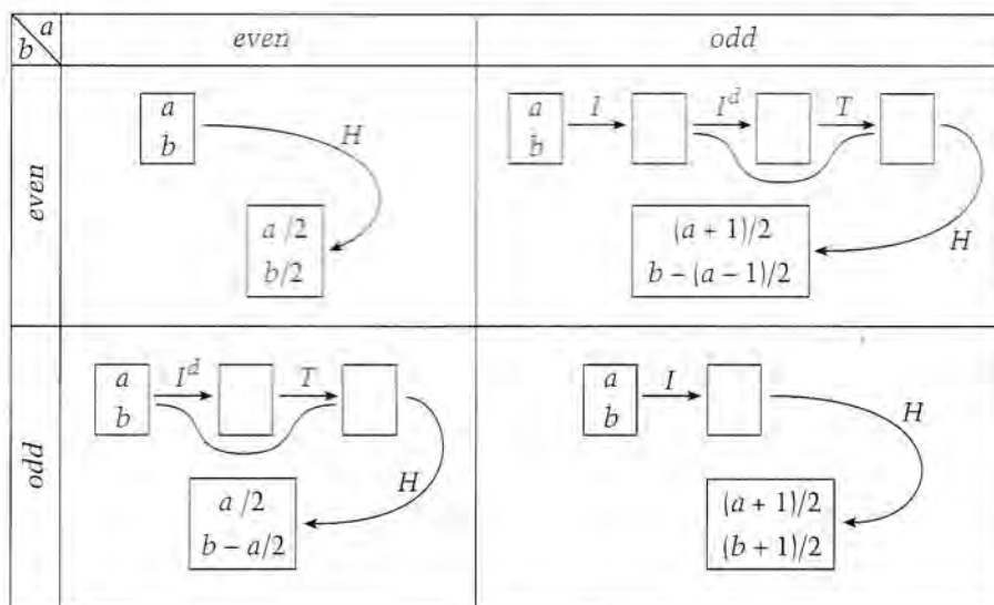
Figure 8. The greater number, b , on the card (a, b) can be decreased (here d = b - a , a > 1 or a = 1 and b is odd).
